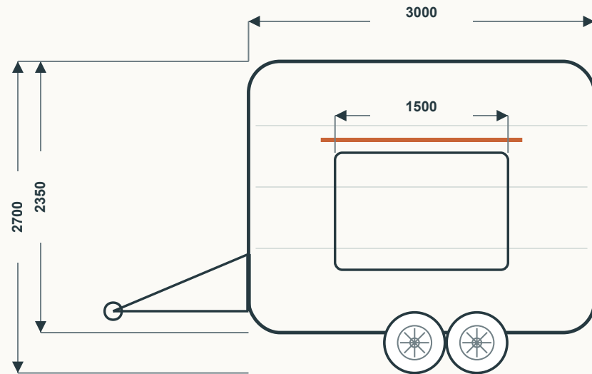
A FACE / SERVING WINDOW SIDE
